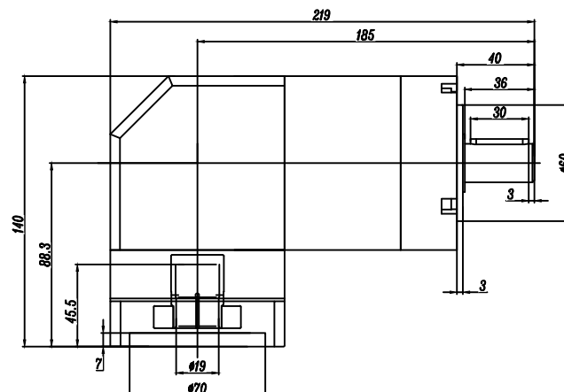
S1光轴:
