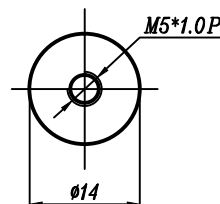
S1光軸:
