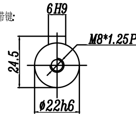
S3孔出:
