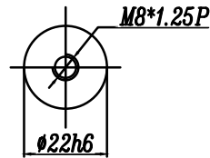
S1光軸:
